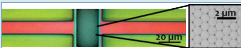
Fig 11 Waveguide and 3D photonic crystals by self-assembly © VTT/ICN
